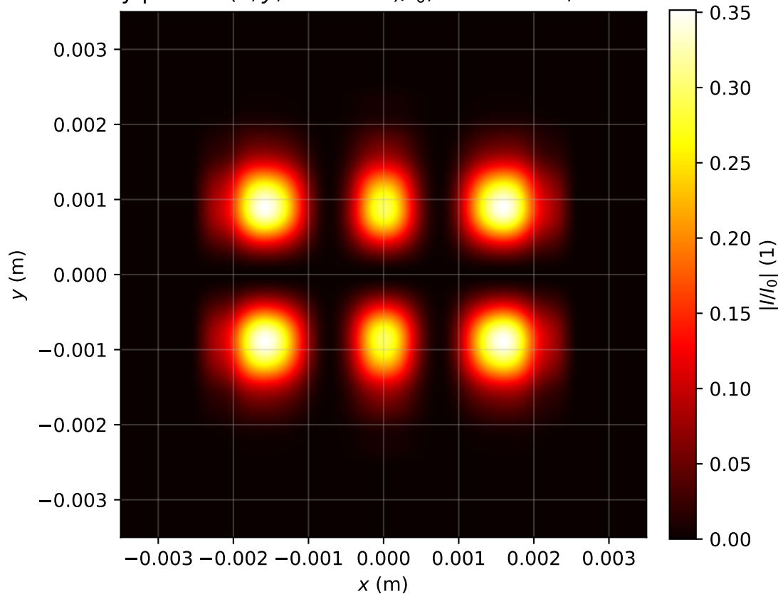
Intensity profile I(x, y, z = 3.423)/I_0 , P_{in}=2.0P_{cr} , artificial time
